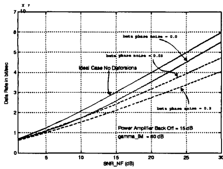
Fig. 2. Achievable data rate for a typical system: the effect of phase noise is expressed by \beta .
