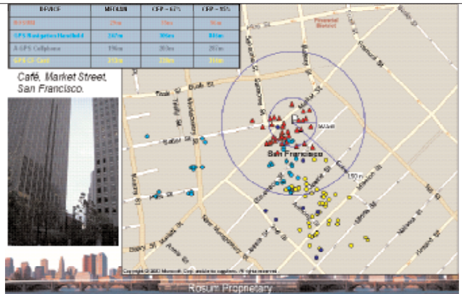
▲ Figure 3 Side-by-side comparison testing with GPS and A-GPS in urban canyons.
